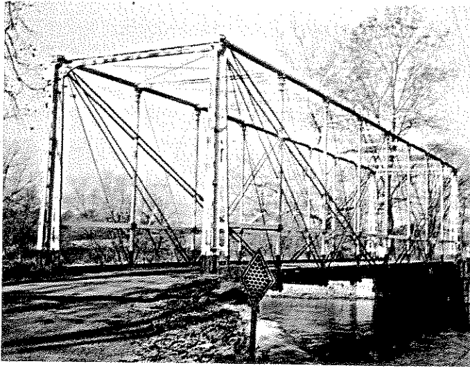
5. Hamden Bridge over Raritan River, Hunterdon County, NJ
