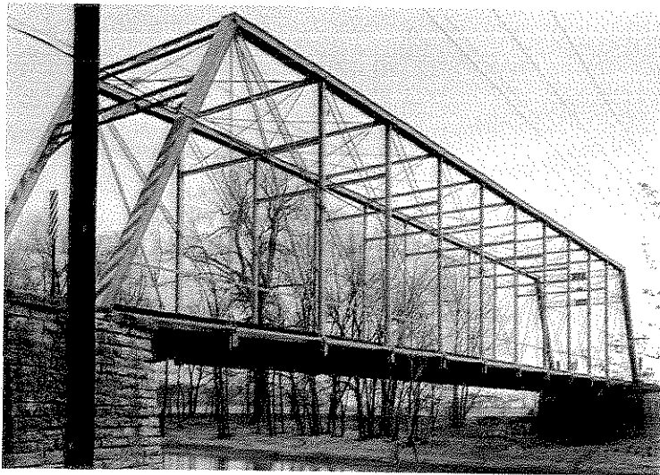
9. Wabash River Bridge, State Rt. 316, Wells County, IN
