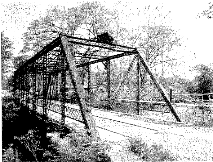
12. Gospel Street Bridge, over Lick Creek, Paoli, IN
