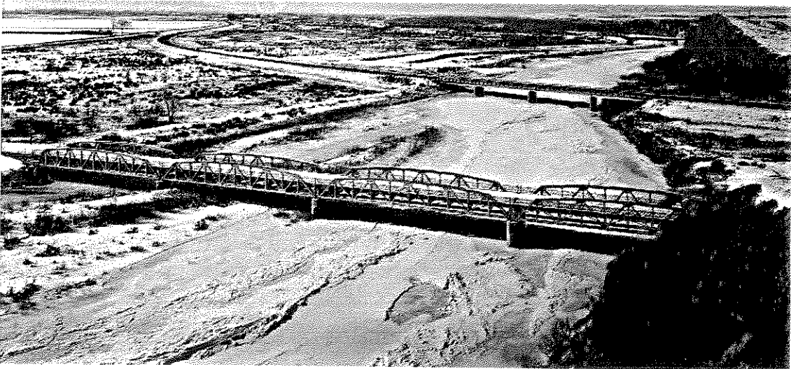
27. Shoshone River Bridge, County Road 111, Big Horn County, WY
