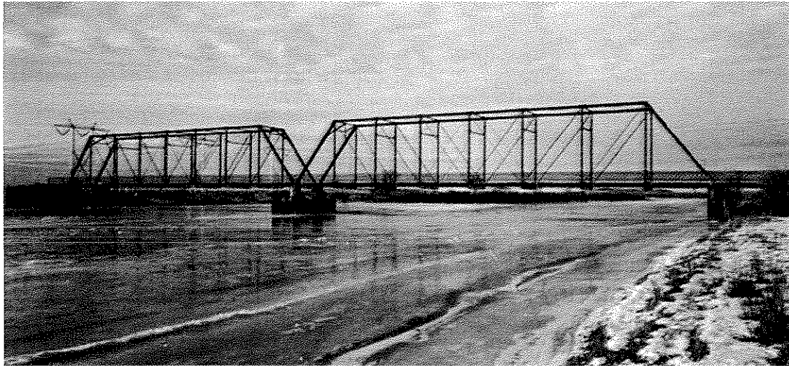
17. Big Island Bridge over Green River, County Road No. 4, Sweetwater County, WY
