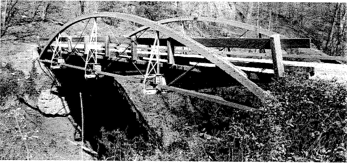
25. Roaring Run Bridge, State Route 657, Bedford County, VA
