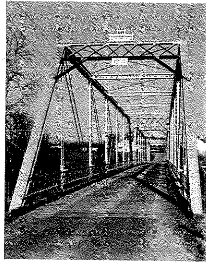
6. State Rt. 256 Bridge over Middle River, Augusta County, VA
