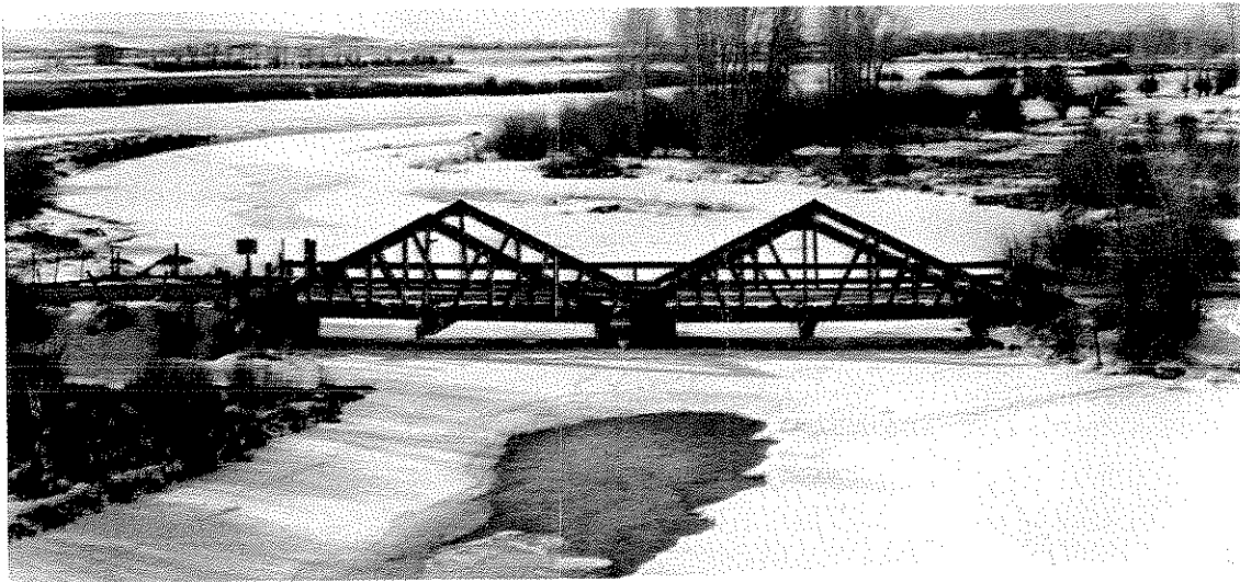
11. New Fork River Bridge, County Rd. 136, Sublette County, WY
