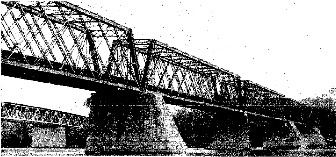
14. Boston & Maine Railroad Bridge, with State Route 9 highway bridge in background, Northampton, MA
